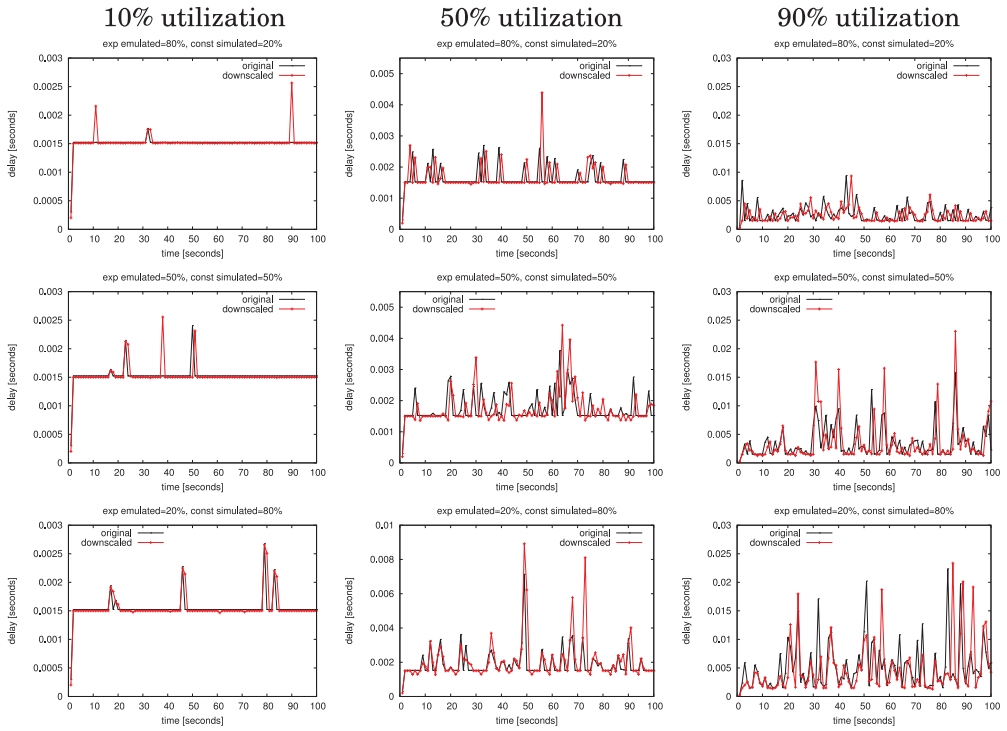
Fig. 7. Packet delays for exponentially distributed emulated flows and constant simulated flows at different utilization levels.
