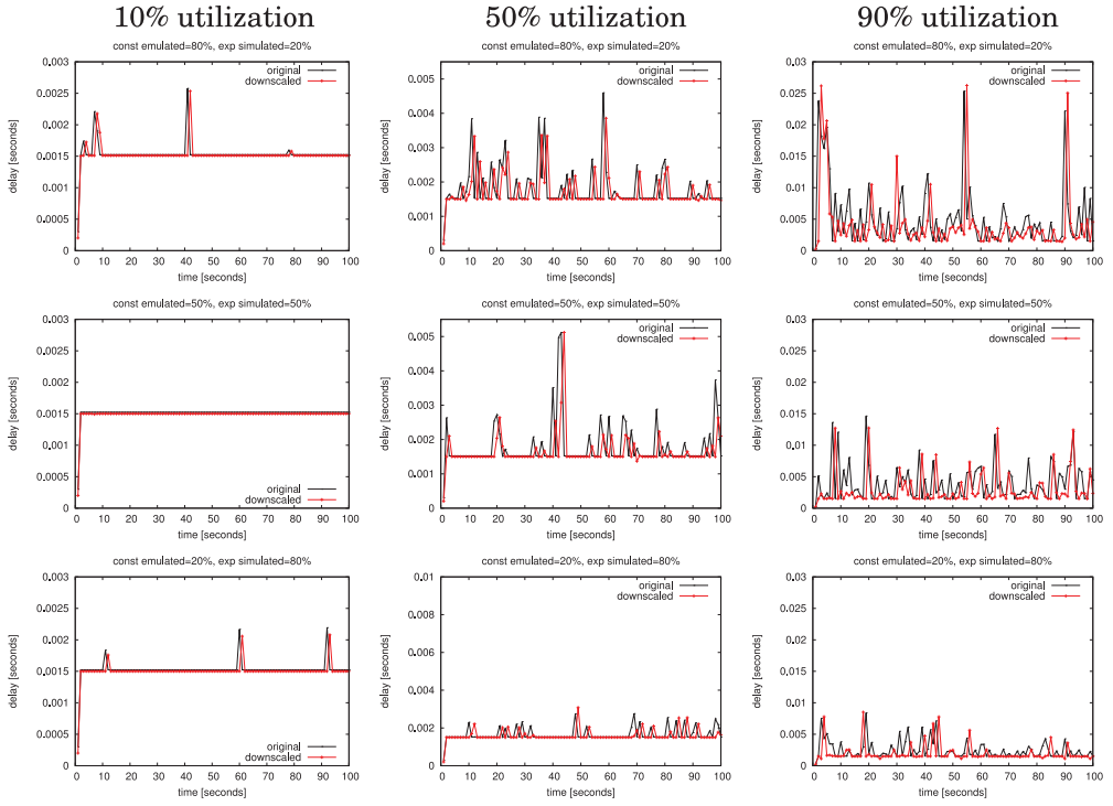
Fig. 6. Packet delays for constant emulated flows and exponentially distributed simulated flows at different utilization levels.
