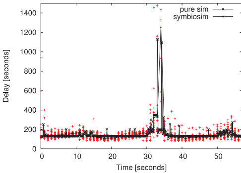
Fig. 11. Round-trip delay.
